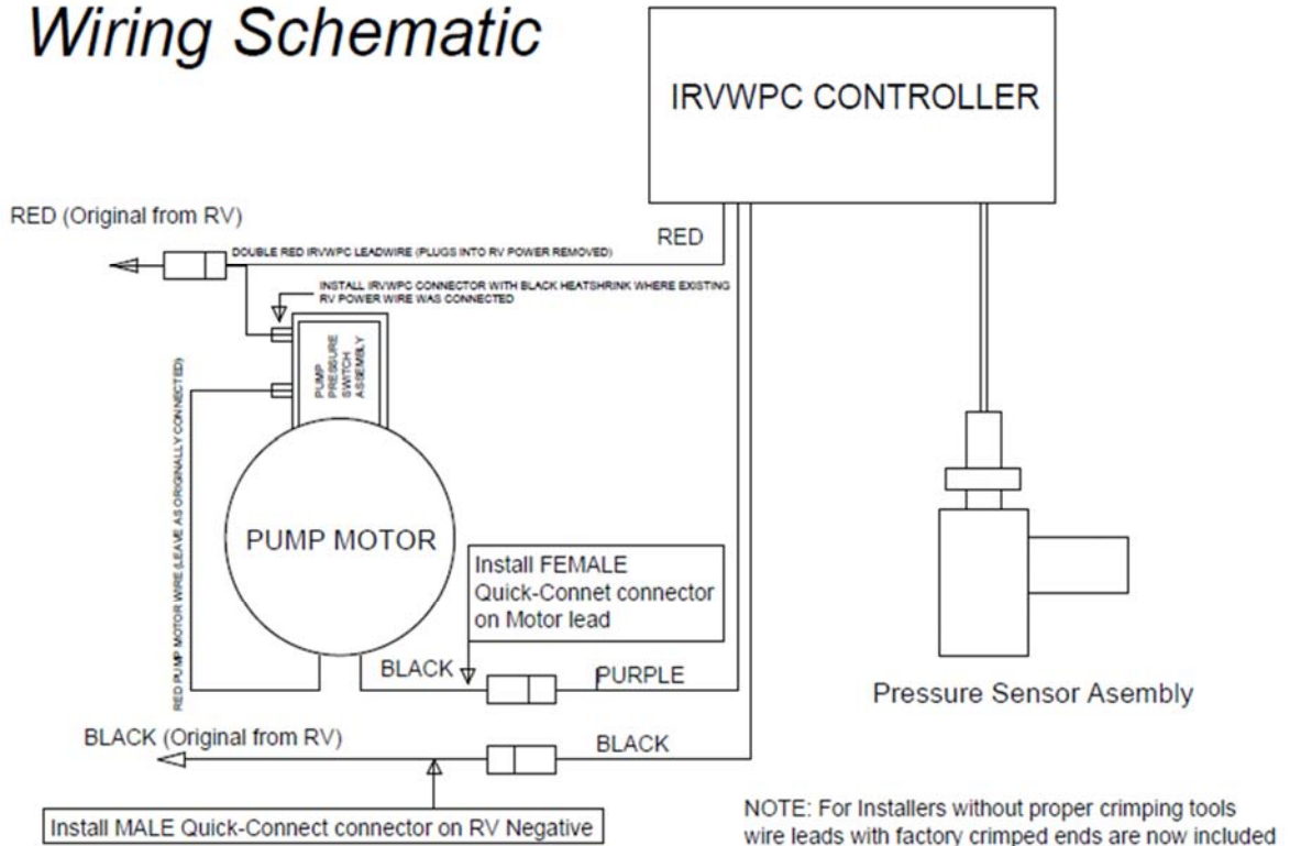
Figure 1: Wiring Schematic
